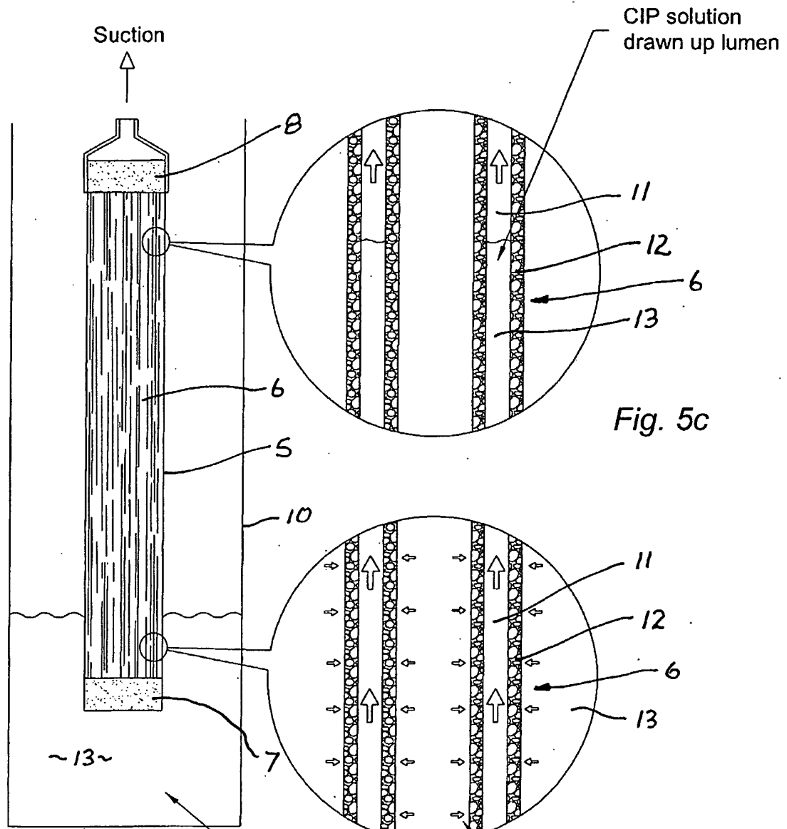
CIP solution drawn through fibre wall and carried up lumen
